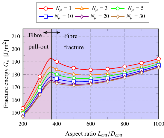
Fig. 8. Estimation of the fracture energy of MWCNT/epoxy composites as a function of the filler aspect ratio, considering different number N_\mu of CNTs agglomerated in bundles.
