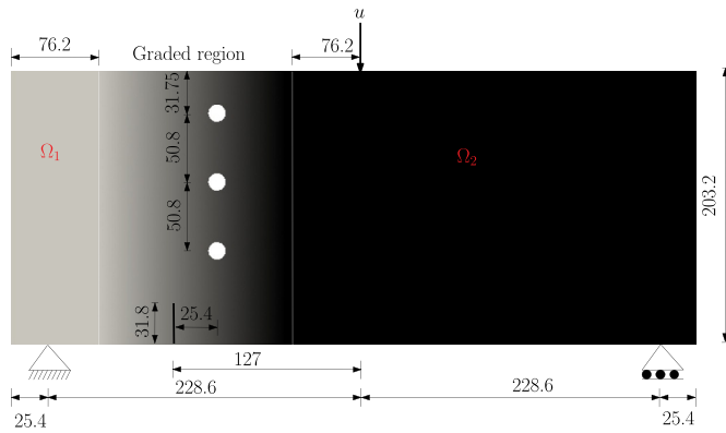
Fig. 9. Geometry and loading configuration, all dimensions are given in mm. The radius of the holes equals 6.35 mm.
