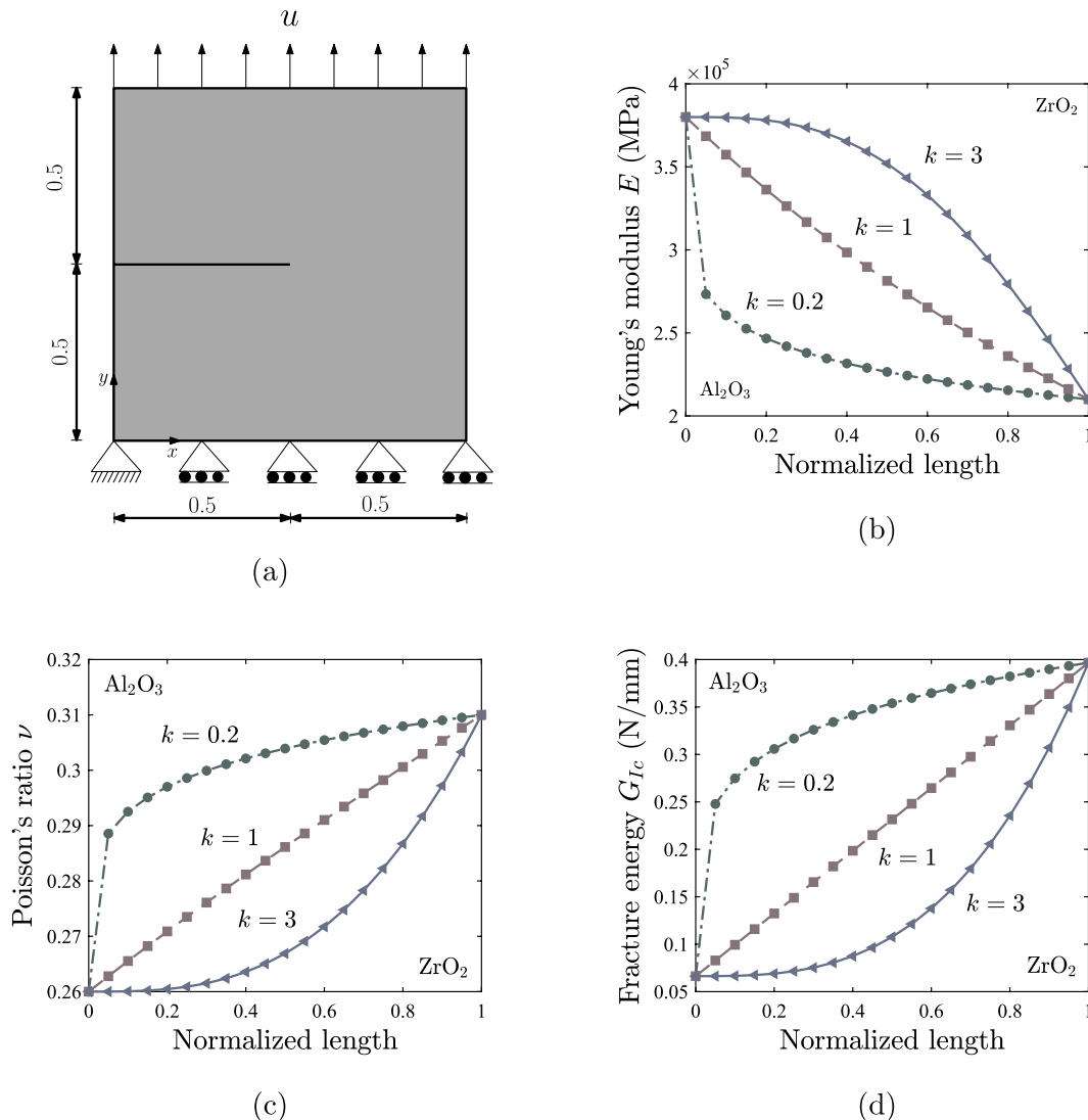
Fig. 1. \text{Al}_2\text{O}_3/\text{ZrO}_2 graded plate, (a) geometry and boundary conditions, with dimensions given in mm, and material property variation for (b) Young's modulus E , (c) Poisson's ratio \nu and (d) critical energy release rate G_c . Normalized lengths 0 and 1 respectively denote 100% \text{Al}_2\text{O}_3 and 100% \text{ZrO}_2 contents.
