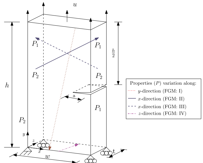
Fig. 11. Geometry, material and loading configuration in a 3D functionally graded specimen. Four cases are considered based on the variation of the elastic and fracture properties.
