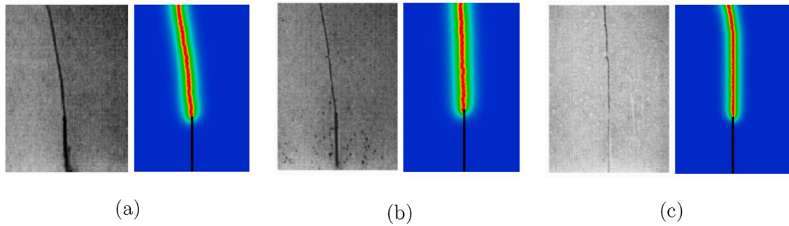
Fig. 7. Epoxy-glass FGMs. Experiments [37] and numerical predictions of crack trajectories for initial crack locations (a) \xi = 0.17 , (b) \xi = 0.58 , and (c) \xi = 1.0 .
