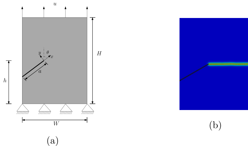
Fig. 4. Edge cracked plate: (a) geometry and boundary conditions, and (b) crack path predicted for the homogeneous case.
