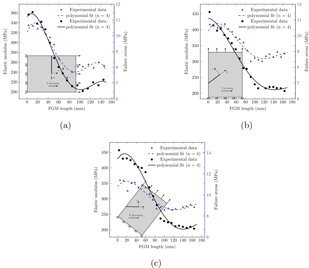
Fig. 3. Geometry and boundary conditions: (a) FGM I, crack perpendicular to material gradient, (b) FGM II, crack at an angle relative to remote loading, and (c) FGM III, crack at an angle relative to remote loading and material gradient at an angle relative to the mode I crack path.
