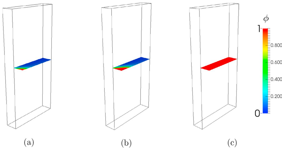
Fig. 13. Crack extension for a graded plate with material properties varying through the thickness (FGM IV) at different loading stages, as given by remote displacements (a) u = 5.137 \times 10^{-3} mm, (b) u = 5.165 \times 10^{-3} mm, and (c) u = 5.177 \times 10^{-3} mm.
