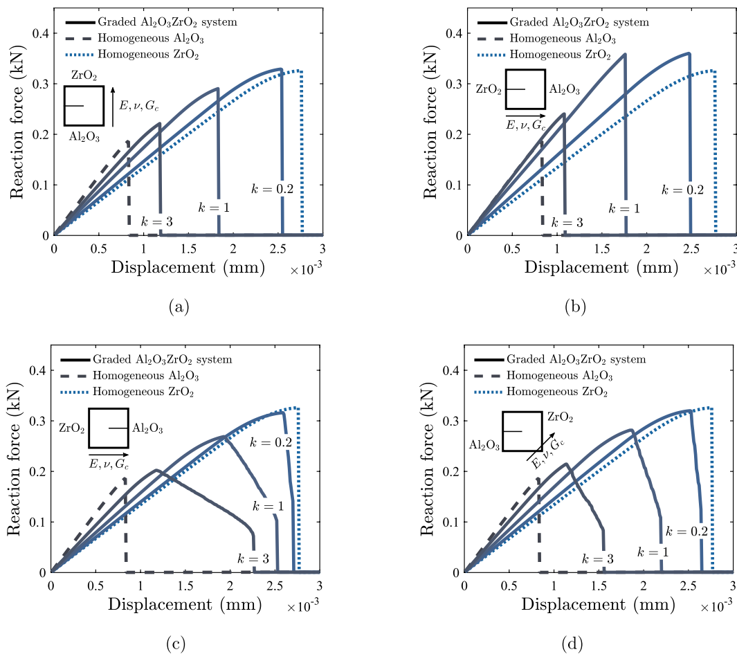
Fig. 2. Load versus displacement curves for material gradation along: (a) the y-axis, (b) the x-axis, with the initial crack on the ZrO 2 side, (c) the x-axis, with the initial crack on Al 2 O 3 side, and (d) with an inclination of 45° relative to the crack.
