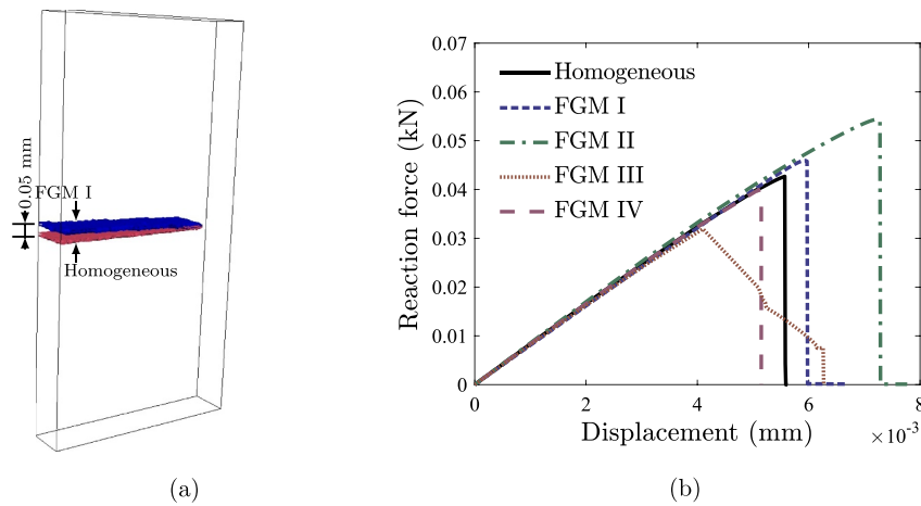
Fig. 12. Three dimensional FGM plate: (a) representative crack trajectories, and (b) load versus displacement curves.
