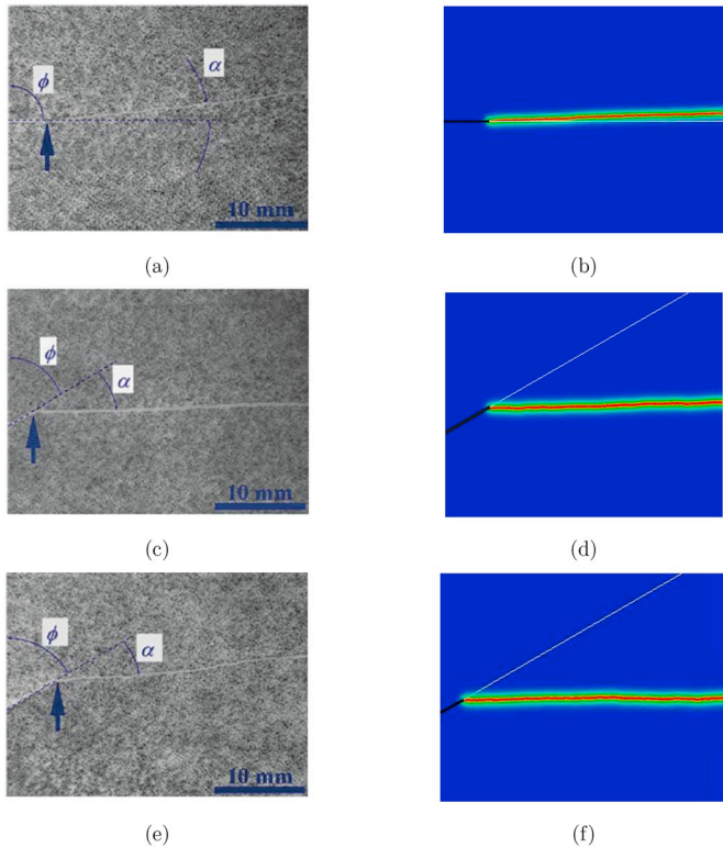
Fig. 5. Numerical predictions of crack propagation paths and comparison with experiments [35]: (a) and (b), FGM I - crack perpendicular to material gradient; (c) and (d), crack at an angle relative to the remote load; and (e) and (f), mode-mixity due to crack inclination and material gradient.
