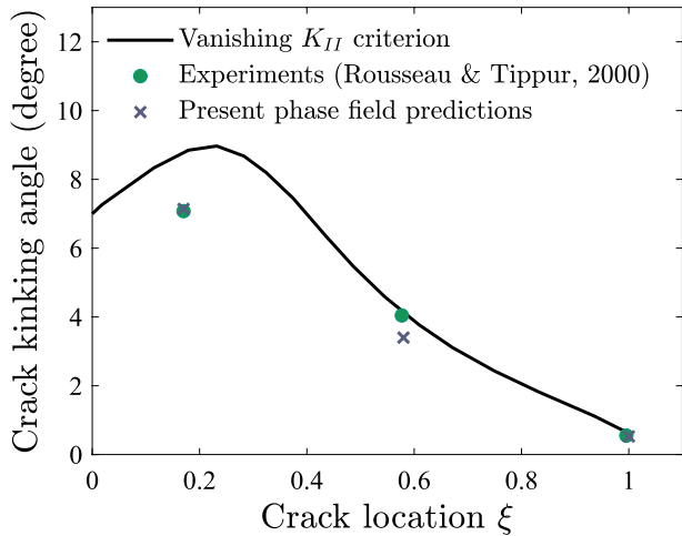
Fig. 8. Epoxy-glass FGMs. Crack kinking angles as a function of the initial crack location along the graded region, \xi .
