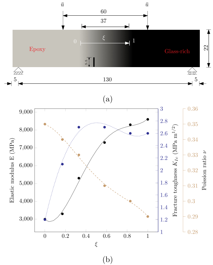
Fig. 6. Four point bending of epoxy-glass FGMs, (a) geometry and boundary conditions (dimensions in mm), and (b) material properties variation.
