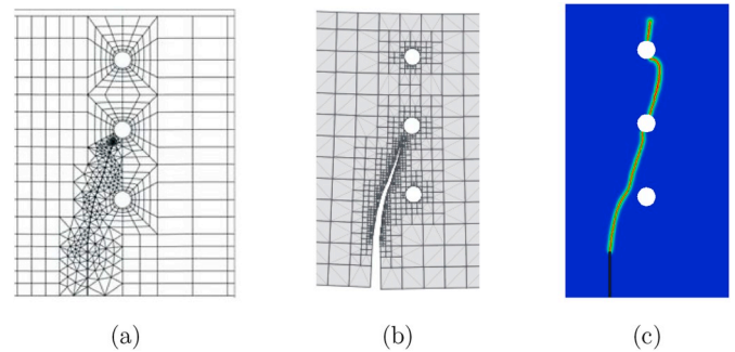
Fig. 10. Complex crack path predictions in functionally graded solids with (a) finite element re-meshing techniques [9], (b) scaled boundary finite element methods [38], and (c) present phase field fracture predictions.
