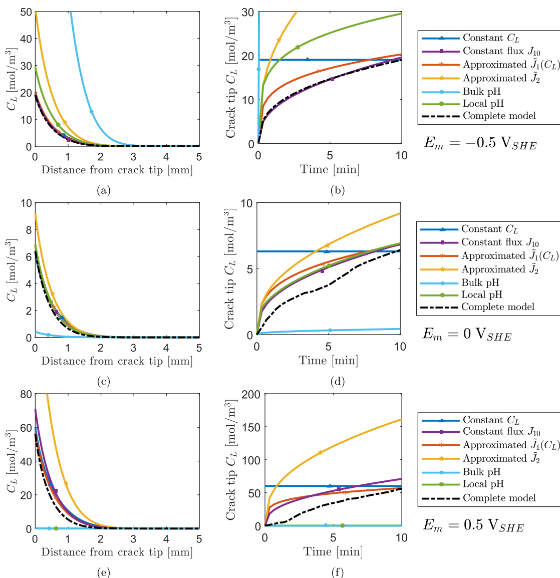
Fig. 18. Assessment of modelling strategies. Lattice hydrogen distribution ahead of the crack after t = 10 min. (left) and evolution of the crack tip lattice hydrogen concentration (right). Seven modelling strategies are considered: (i) prescribing a constant hydrogen concentration, (ii) prescribing a constant hydrogen flux, (iii) our approximated flux model \tilde{J}_1 , (iv) our further simplified flux model \tilde{J}_2 , two cases where the electrochemistry is not solved for upon the assumption that the pH is known, one using the bulk pH (v) and another one using the local one (vi), and (vii) our complete electro-chemo-mechanical model (the reference result). Results are shown for three values of the applied potential: E_m = -0.5 V_{SHE} (a & b), E_m = 0 V_{SHE} (c & d) and E_m = 0.5 V_{SHE} (e & f). Based on the assumptions discussed and Fig. 17, the values used are: C_L = 19 \text{ mol/m}^3 , \tilde{J}_2 = 1.1 \cdot 10^{-4} \text{ mol/(m}^2 \text{ s)} , J_{10} = 4.2 \cdot 10^{-5} \text{ mol/(m}^2 \text{ s)} , and local pH= 13 ( E_m = -0.5 V_{SHE} ); C_L = 6.3 \text{ mol/m}^3 , \tilde{J}_2 = 2.0 \cdot 10^{-5} \text{ mol/(m}^2 \text{ s)} , J_{10} = 1.5 \cdot 10^{-5} \text{ mol/(m}^2 \text{ s)} , and local pH= 3.7 ( E_m = 0 V_{SHE} ); C_L = 60 \text{ mol/m}^3 , \tilde{J}_2 = 3.4 \cdot 10^{-4} \text{ mol/(m}^2 \text{ s)} , J_{10} = 1.5 \cdot 10^{-4} \text{ mol/(m}^2 \text{ s)} , and local pH= 1.6 and ( E_m = 0.5 V_{SHE} ).
