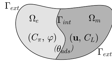
Fig. 1. Schematic overview of the electrolyte and metal domains, and (in brackets) the degrees of freedom used to describe the electrochemical phenomena relevant to each of them.
