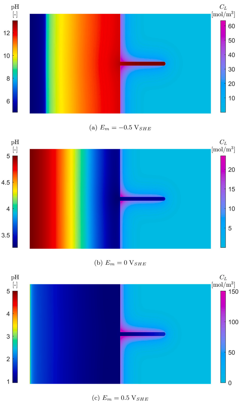
Fig. 8. Metal–electrolyte interactions: influence of the applied potential E_m . Contours of pH (left, electrolyte domain) and lattice hydrogen concentration (right, metal domain) at a time t = 10 \text{ min} for the following metal potentials: (a) E_m = -0.5 \text{ V}_{SHE} , (b) E_m = 0 \text{ V}_{SHE} , and (c) E_m = 0.5 \text{ V}_{SHE} .
