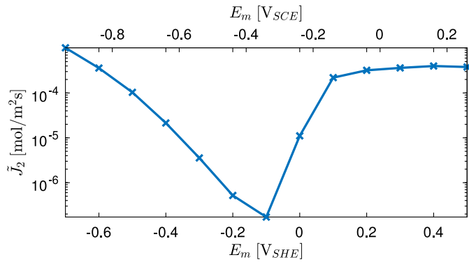
Fig. 17. Hydrogen entry rate estimated from the simplified model shown in Eq. (53) and the environmental conditions given in Fig. 16. The results correspond for the case of a sufficiently large crack, after a time of t = 10 min, neglecting the fluid velocity and prescribing a pH of 5 and a potential of \varphi = 0 V SHE at the external electrolyte edge (located at 10 mm from the metal surface). Other parameters used k_{v_a} = 10^{-4} m/s, k_{v_b} = 10^{-8} m/s and \alpha = 0.5 .
