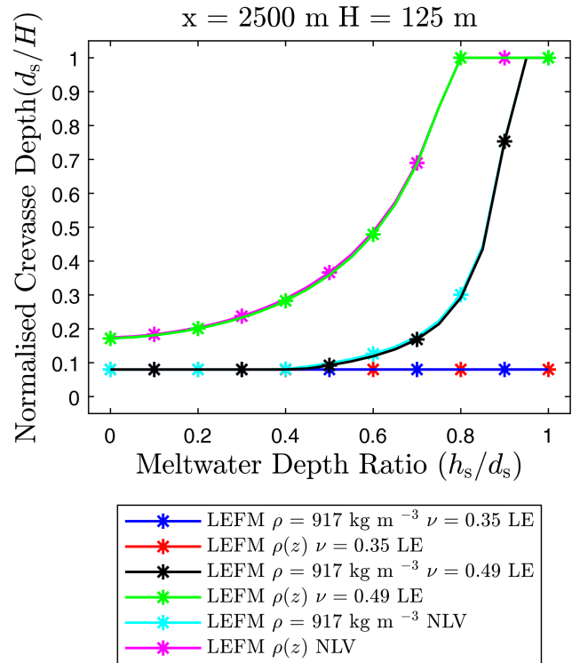
Figure 11. Normalized crevasse depth predictions versus meltwater depth ratio for a single isolated surface crevasse located in the far-field region ( x = 2500\text{ m} ) considering a linear elastic (LE) and non-linear viscous (NLV) rheology.
