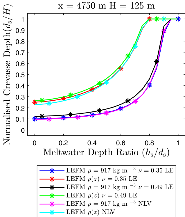
Figure 10. Normalized crevasse depth predictions versus meltwater depth ratio for a single isolated surface crevasse located close to the ice shelf front ( x = 4750\text{ m} ) considering a linear elastic (LE) and non-linear viscous (NLV) rheology.
